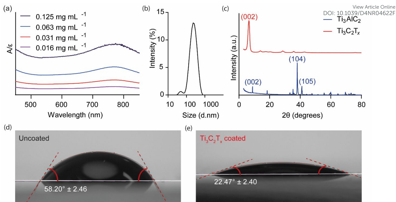
Fig. 1 – Physical characterisation of \text{Ti}_3\text{C}_2\text{T}_x . (a) UV-Vis spectroscopy of \text{Ti}_3\text{C}_2\text{T}_x solutions of varying concentrations normalised to the molar extinction coefficient ( \epsilon = 29.78 \text{ L g}^{-1} \text{ cm}^{-1} ) calculated from the calibration curve (ESI Fig 5). (b) Dynamic light scattering was used to determine the particle size and distribution of the \text{Ti}_3\text{C}_2\text{T}_x solution. (c) X-ray diffraction comparing the crystal structure of \text{Ti}_3\text{AlC}_2 to the synthesised and vacuum-filtered \text{Ti}_3\text{C}_2\text{T}_x film (Cu K_\alpha radiation source ( \lambda = 1.5406 \text{ \AA} ) at 40 kV and 15 nA beam current). (d) The contact angle of the uncoated ( 58.20 \pm 2.46^\circ ) and (e) \text{Ti}_3\text{C}_2\text{T}_x coated ( 22.47 \pm 2.40^\circ ) glass slide surface.
