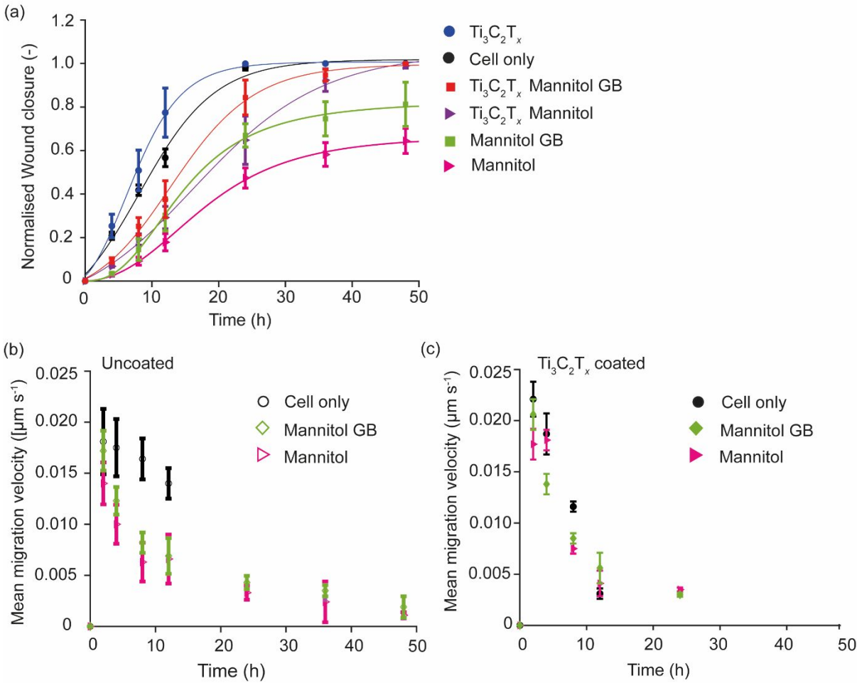
Fig. 2 – Cell migration scratch assay results indicating a significant reduction in keratocyte migratory capacity under mannitol-induced, hyperosmotic stress conditions and a significant protective effect for cells grown on Ti_3C_2T_x coatings to more rapidly close the scratch, (a) Normalised wound closure (WC) over time, comparing keratocyte scratch closure under iso-osmotic conditions to scratch closure under hyperosmolar conditions in the presence and absence of Ti_3C_2T_x coatings and GB. Across all cases, the curve fit yielded an R^2 value >0.99 . (b) Mean migration velocity (MV) of cells over time under normal iso-osmolarity (cell-only), mannitol-induced hyperosmolarity (mannitol), and mannitol-induced hyperosmolarity with GB (mannitol GB) in uncoated and (c) Ti_3C_2T_x coated conditions, ( n=3 , mean \pm SD).
